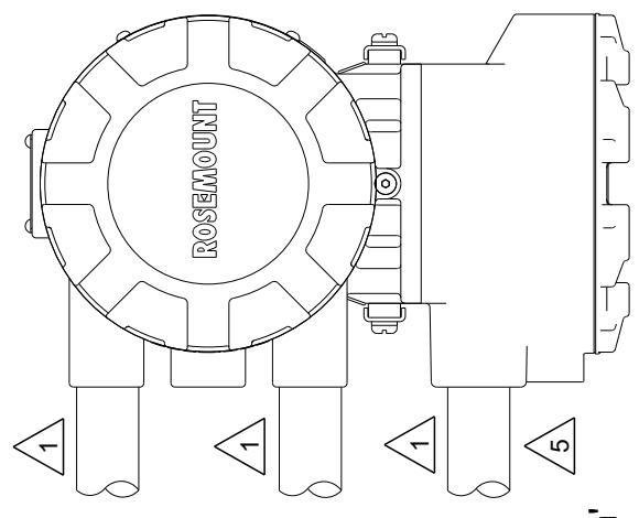
MODEL 8732EM REMOTE MOUNT NC OPTION
