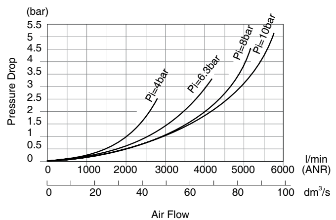
High Flow St. steel filter 3/4" NPT Ref. : 342A920D Filtration 25 μm with P inlet 4 - 6.3 - 8 - 10 bar
