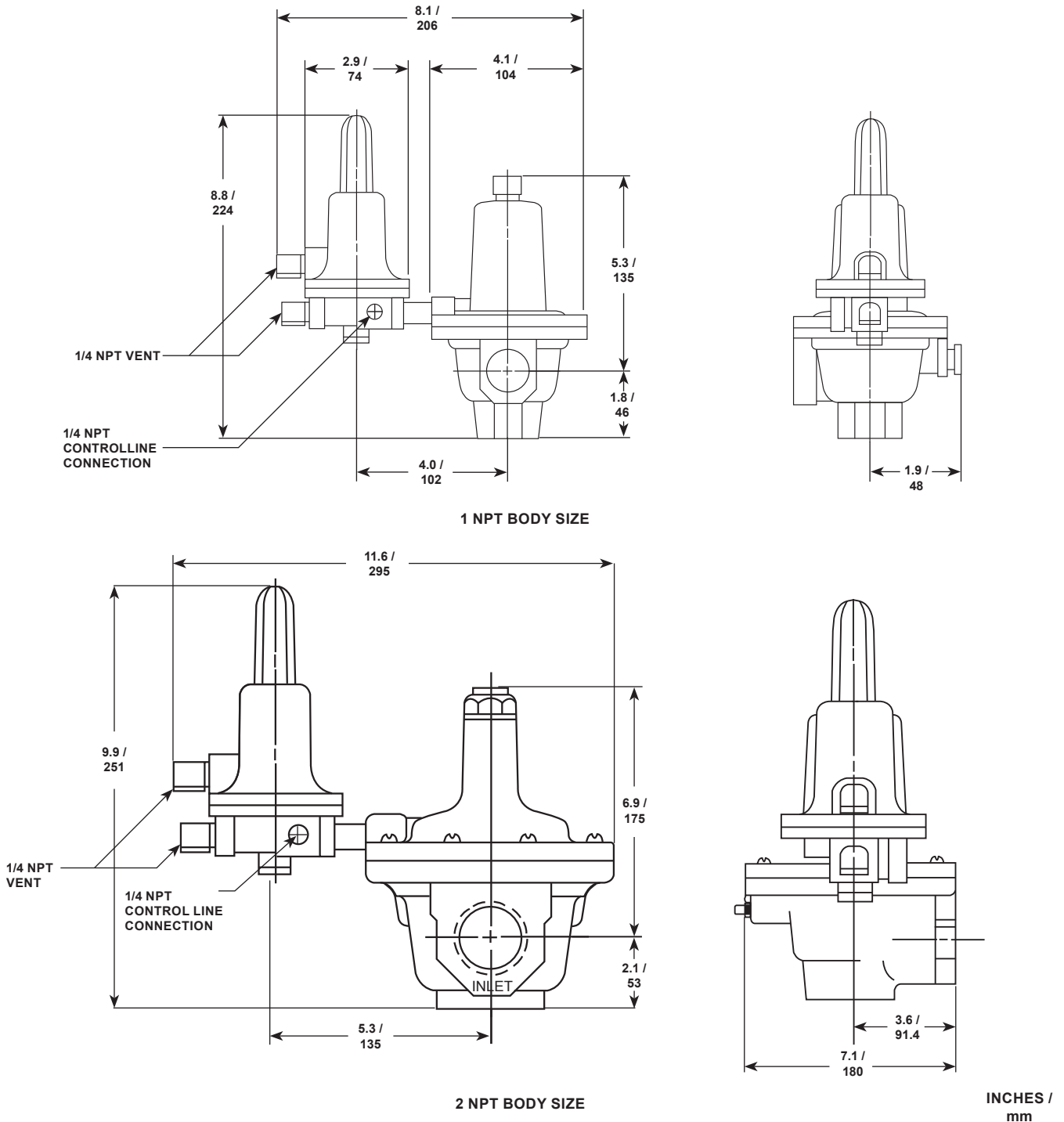
Figure 4. Dimensions
