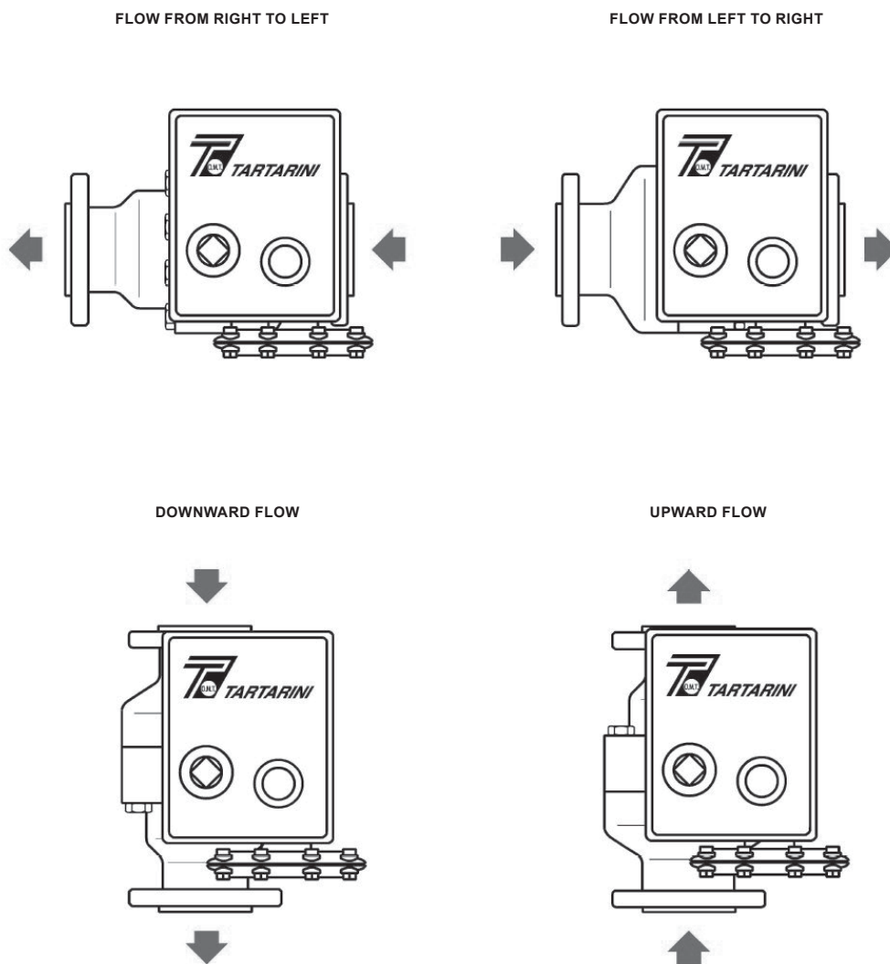
Figure 3. Type BM5A Slam-Shut Valve Flow Orientation
