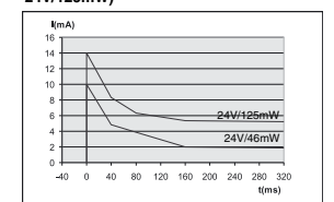
Grafico corrente/tempo (24V/46mW - 24V/125mW) Stroom-tijdsdiagram (24V/46mW - 24V/125mW)
