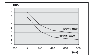
Strøm-tid diagram (12V/12mW - 12V/32mW) Ström-tidtabell (12V/12mW - 12V/32mW) Virta-aikakaavio (12V/12mW - 12V/32mW)
