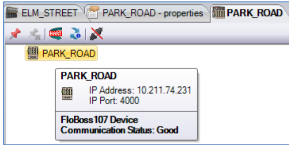
Figure 3-26. Active Connection Pane
