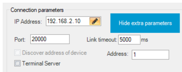
Figure 3-16. IP Connection Settings – FB1000/FB2000 Series Flow Computers & FB3000 RTUs
