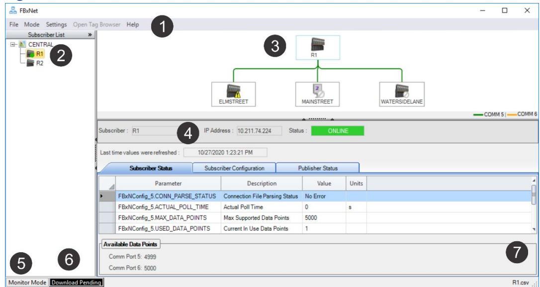
Figure 4-12. FBx Main Screen
