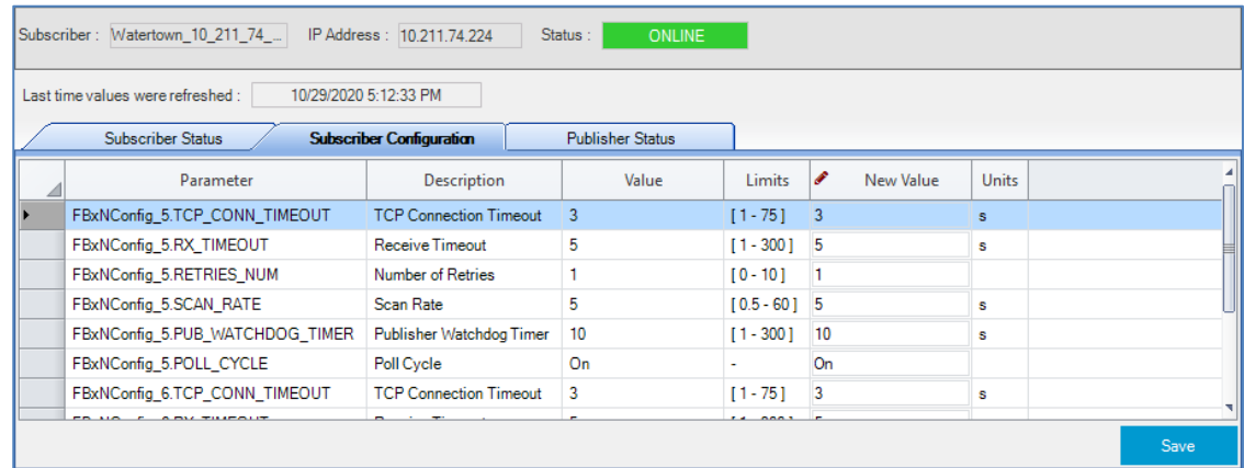
Figure 4-25. Subscriber Configuration tab
