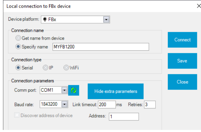
Figure 5-11. Creating a Connection to the Flow Computer
