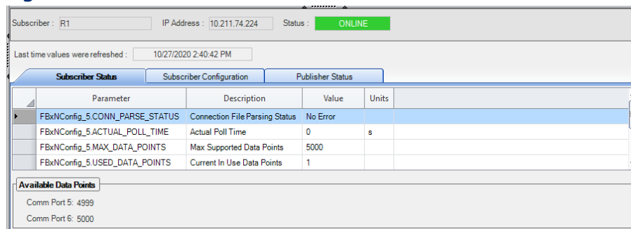
Figure 4-22. FBxNet – Subscriber Status tab visible
