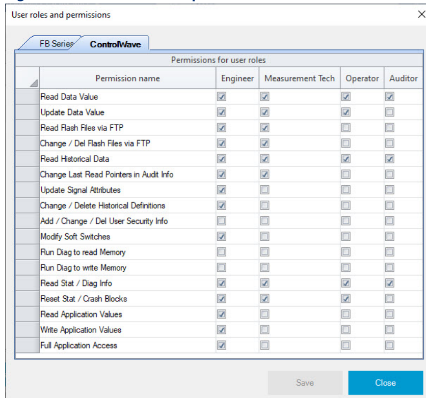
Figure 5-16. User roles and permissions-ControlWave
