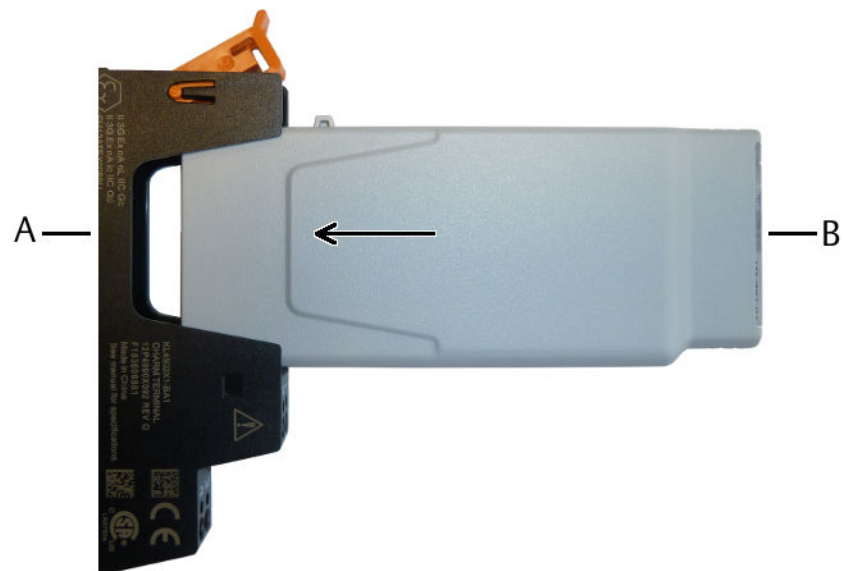
Figure 3-2: CHARM installation
