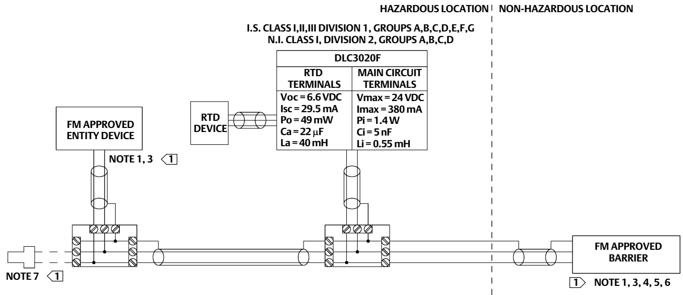
Figure 1. FM Schematic – Drawing GE37117 (Refer to figure 2 for Notes)
