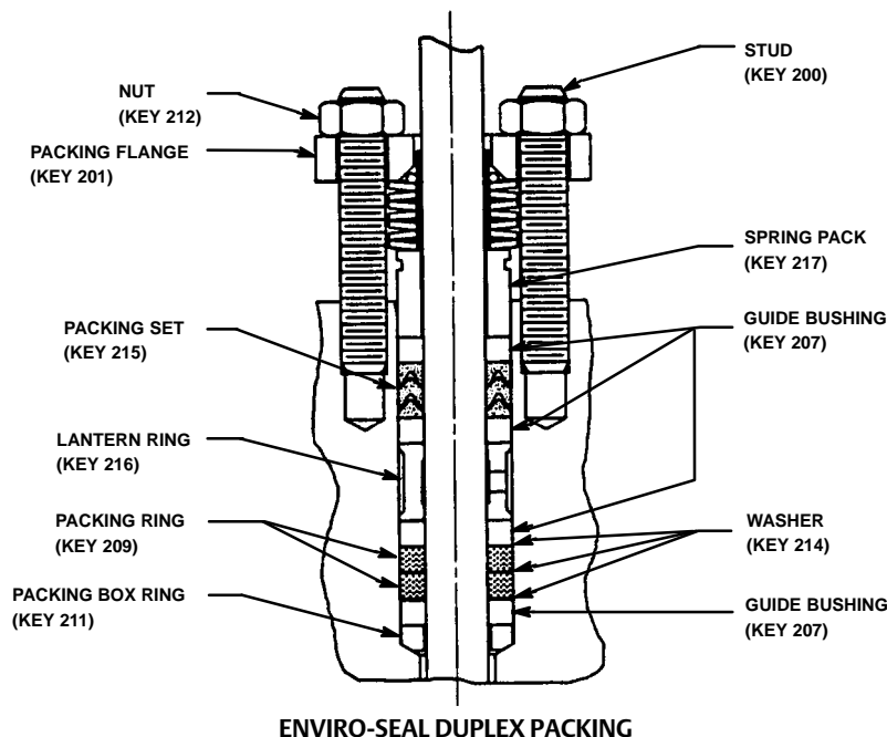
ENVIRO-SEAL DUPLEX PACKING
