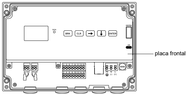
Fig. 2.1: Transmisor FLUXUS G532CA
