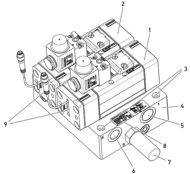
Geräteübersicht Materialnummer R422003729, -730, -980, -982 | Vue d'ensemble de l'appareil références R422003729, -730, -980, -982 | Device overview, material number R422003729, -730, -980, -982 | Panoramica dell'apparecchio R422003729, -730, -980, -982 | Vista general del aparato n.º de material R422003729, -730, -980, -982 | Enhetsöversikt materialnummer R422003729, -730, -980, -982
