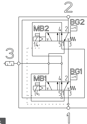
Schaltbild Varianten R422003730, -982, interne Vorsteuerung (links) und R422003729, -980, externe (rechts) Vorsteuerung | Schéma pneumatique variantes R422003730, -982, pilotage interne (gauche) et R422003729, -980, pilotage externe (droite) | Wiring diagram for variants R422003730, -982, internal pilot (left) and R422003729, -980, external pilot (right) | Varianti schema di collegamento R422003730, -982, pilotaggio interno (a sinistra) ed R422003729, -980 pilotaggio esterno (a destra) | Diagrama de conexiones variantes R422003730, -982, pilotaje previo interno (izquierda) y R422003729, -980 pilotaje previo externo (derecha) | Kopplingsschema varianter R422003730, -982, intern pilotmatning (vänster) och R422003729, -980, extern pilotmatning (höger)
