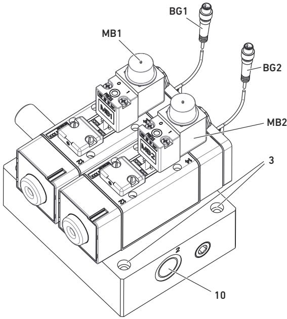
Geräteübersicht Materialnummer R422003729, -730, -980, -982 | Vue d'ensemble de l'appareil références R422003729, -730, -980, -982 | Device overview, material number R422003729, -730, -980, -982 | Panoramica dell'apparecchio R422003729, -730, -980, -982 | Vista general del aparato n.º de material R422003729, -730, -980, -982 | Enhetsöversikt materialnummer R422003729, -730, -980, -982
