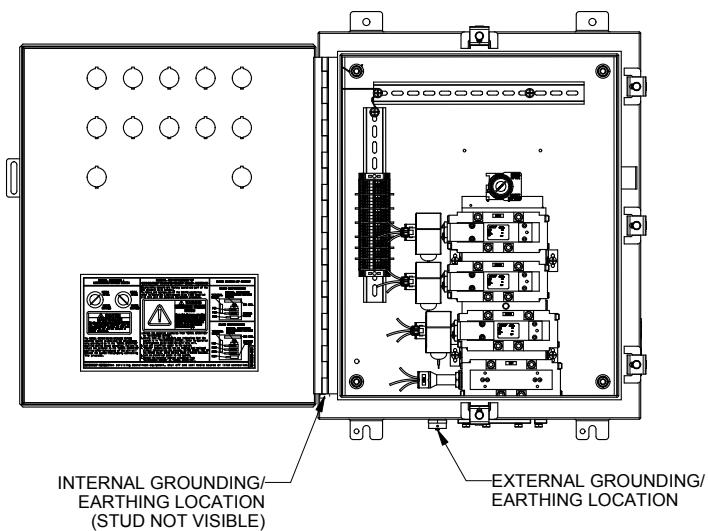
Figure 3C. Grounding Connections
