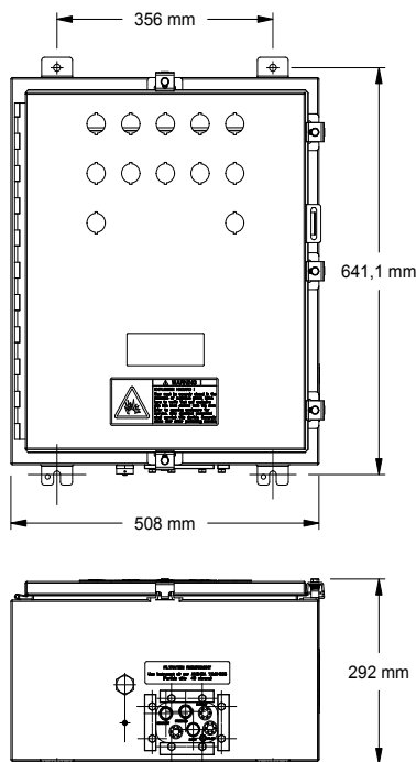
Figure 2. Mounting Dimension
