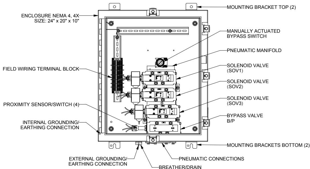
Figure 1A. RCS 2003D With Enclosure Components Approx Weight 48.2 kg (106 lbs.)
