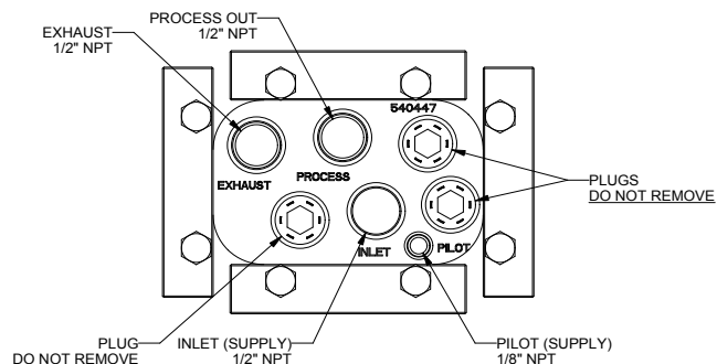
Figure 3A. Pneumatic Connections
