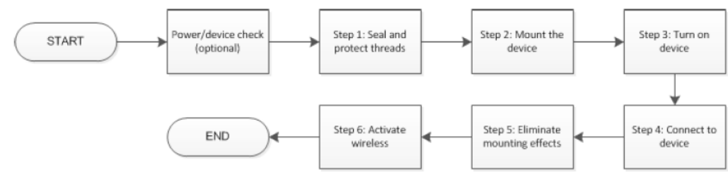
Figure 3-2: Installation Flowchart
