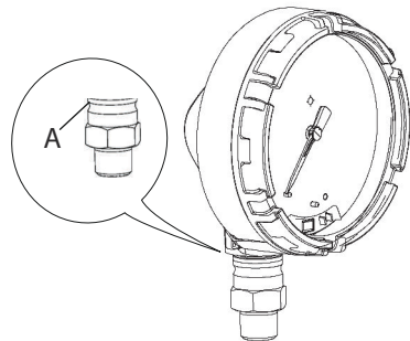
Figure 3-4: Low Side Pressure Port
