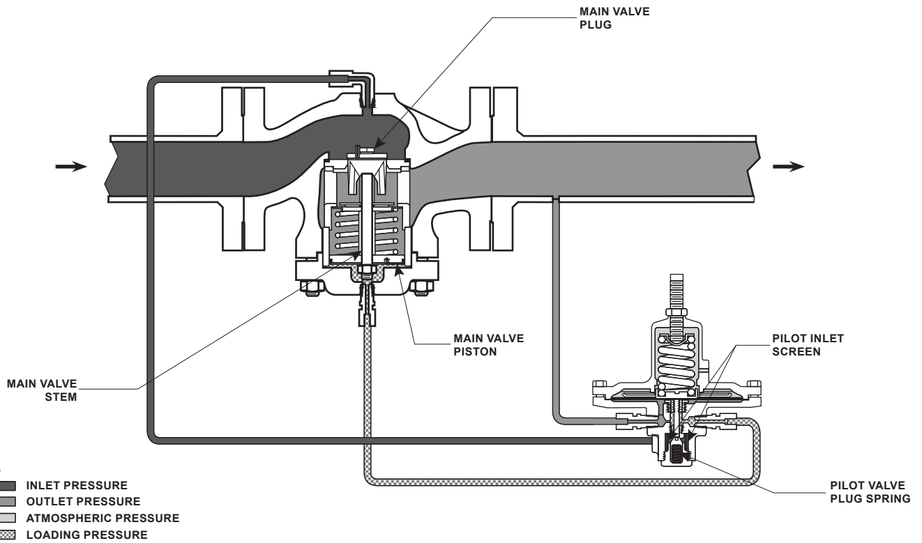
Figure 2. Type 92S Pilot-Operated Steam Regulator Operational Schematics
