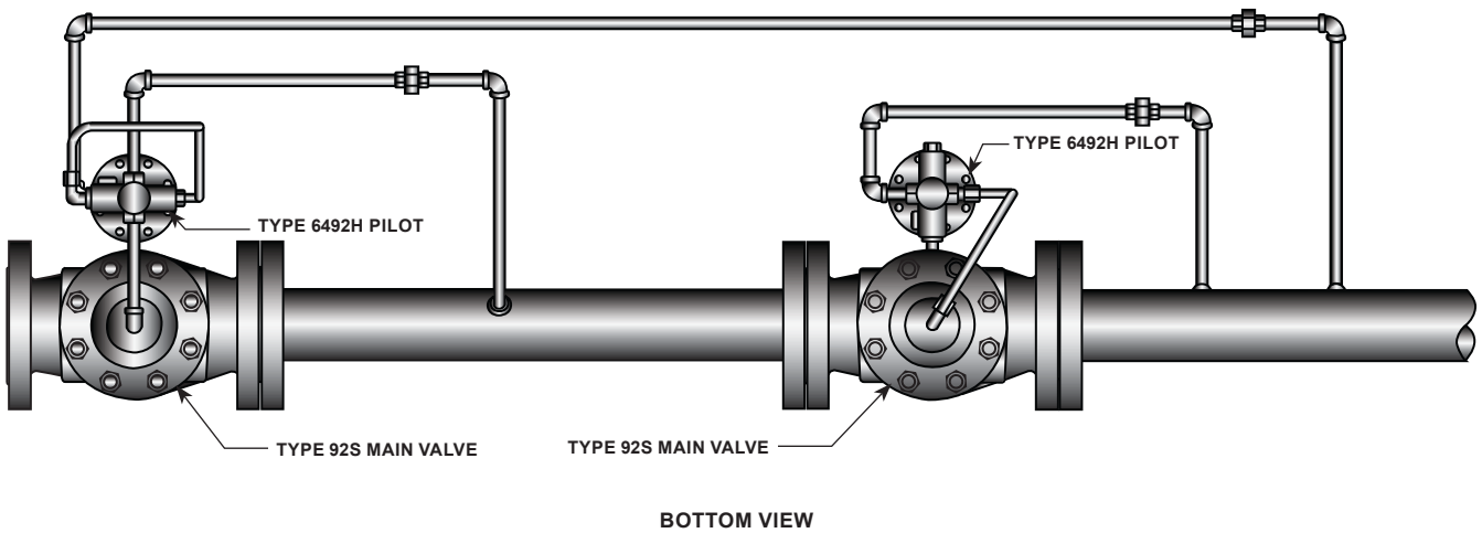
BOTTOM VIEW
