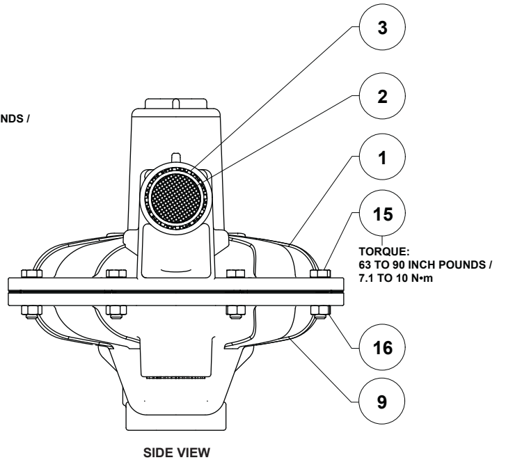
MAIN VALVE
