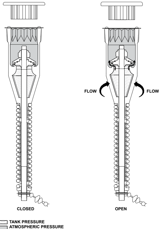
Figure 2. Operational Schematic
