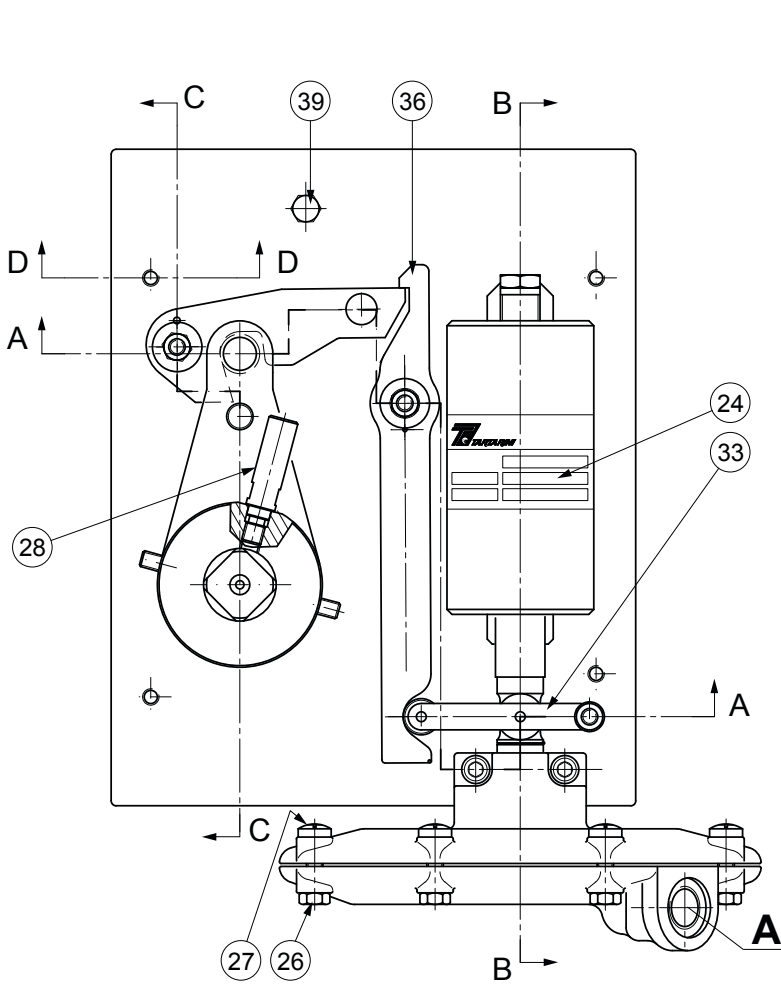
Figure 8. OS/80X Series Slam-Shut Controller Assembly (Standard Version) (continued)
