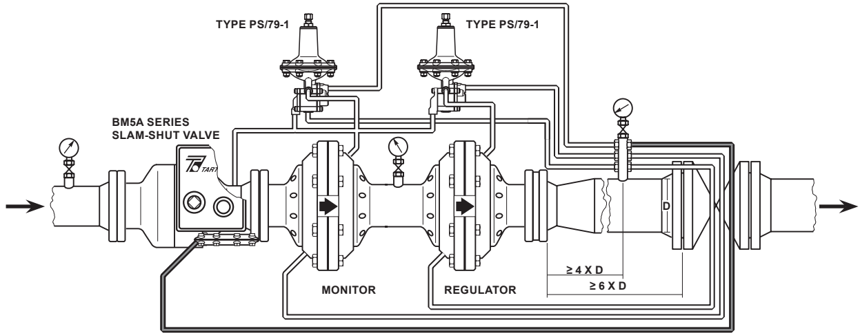
SLAM-SHUT VALVE WITH OS/80X SERIES CONTROLLER - INSTALLATION IN A LOW PRESSURE REGULATING LINE
