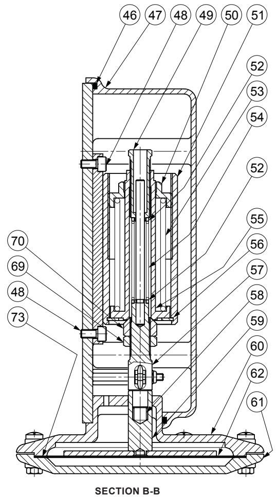
Figure 8. OS/80X Series Slam-Shut Controller Assembly (Standard Version) (continued)
