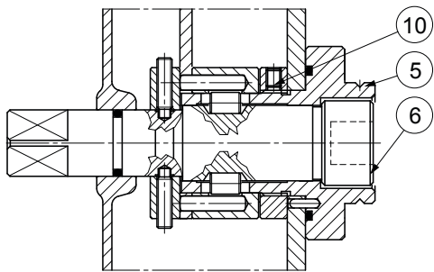
DETAIL OF TYPE OS/80X-R REINFORCED FOR TYPE BM5A DN 150 / NPS 6
