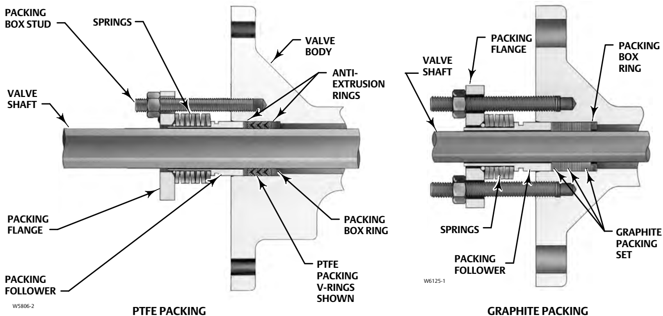
Figure 4. Optional ENVIRO-SEAL Packing Arrangements
