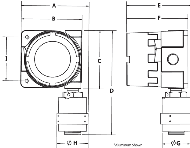
Figure 1 - Millennium II M21 Single Channel Transmitter Dimensions
