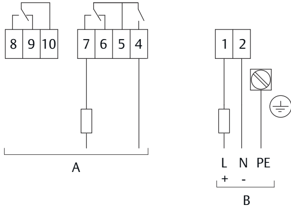
Figure 3: Terminal Block Connections for Safety Function
