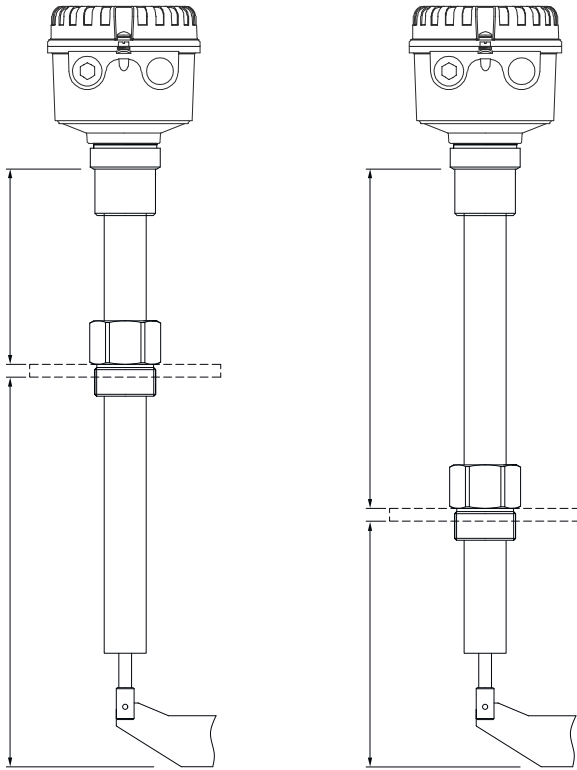
Figure 20: Sliding Sleeve
