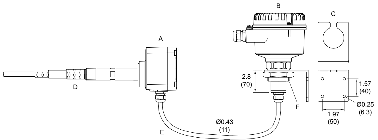
Figure 2: Rosemount 2555 Remote Version
