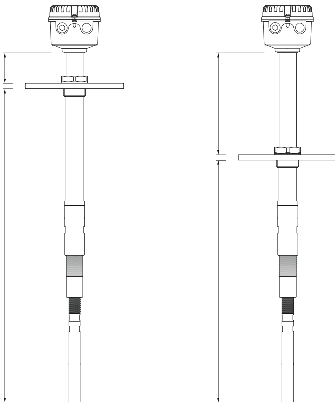
Figure 9: Sliding Sleeve
