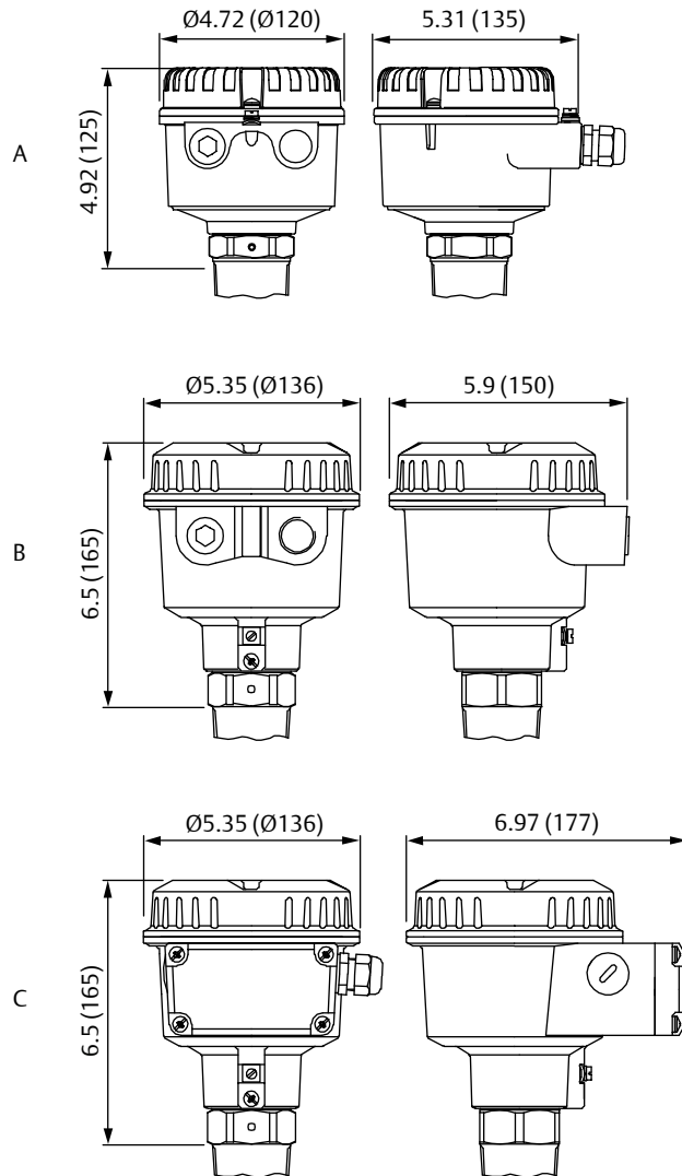
Figure 1: Rosemount 2555 Housing Options
