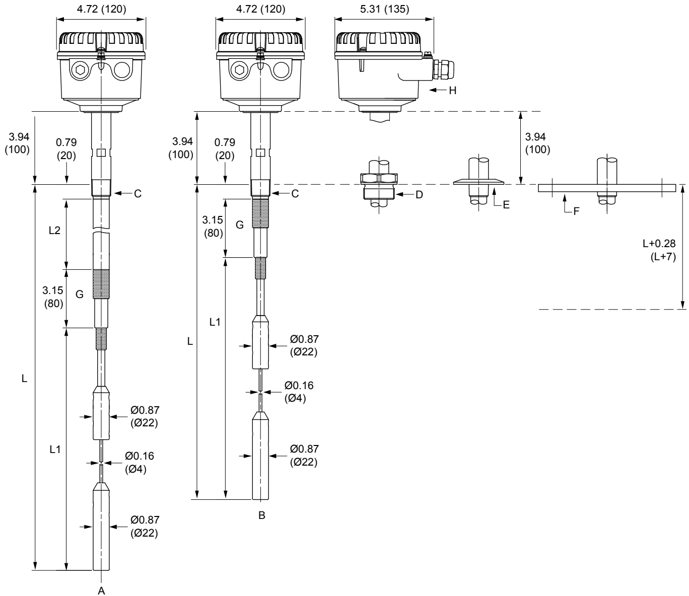
Figure 4: Rosemount 2555 Capacitance Probe Level Switch (Thermal Profile code R)
