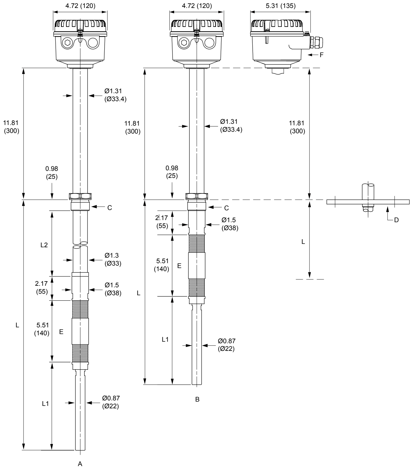
Figure 7: Rosemount 2555 Capacitance Probe Level Switch (Thermal Profile code E)
