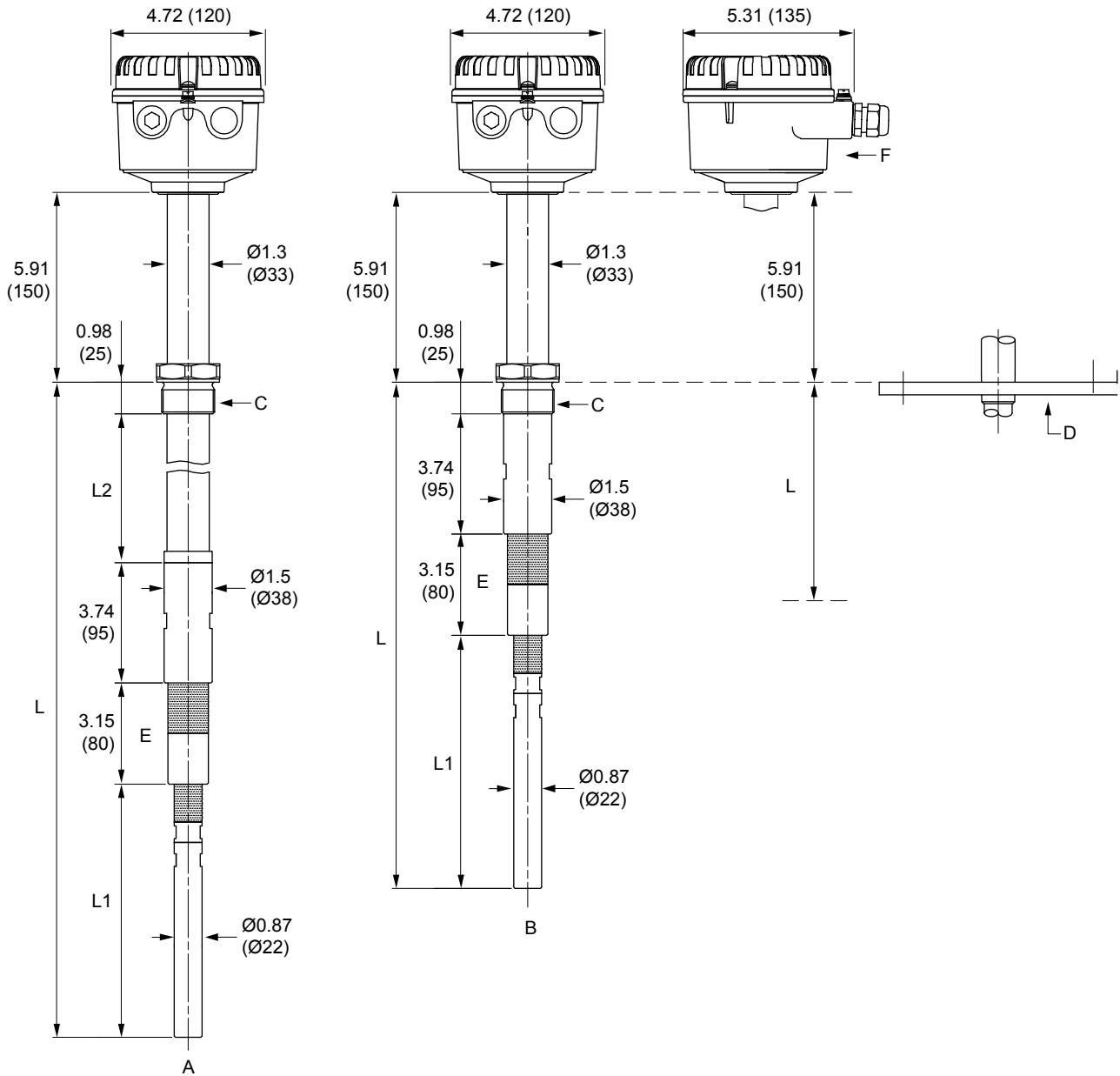
Figure 5: Rosemount 2555 Capacitance Probe Level Switch (Thermal Profile code M)
