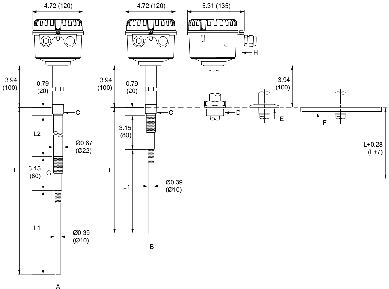
Figure 3: Rosemount 2555 Capacitance Probe Level Switch (Thermal Profile code S)
