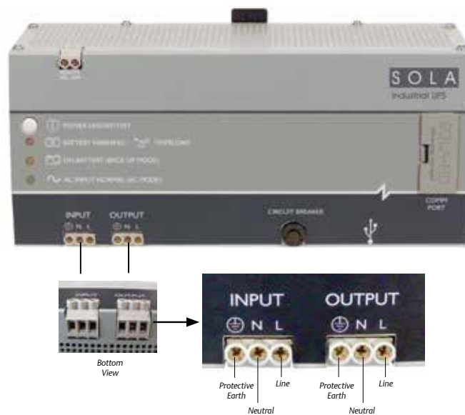
Figure 2: Input/Output Terminals
