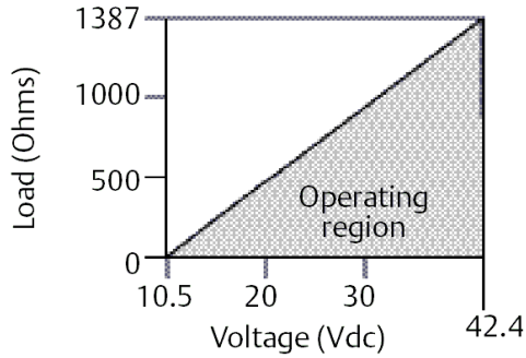
Figure 3-3: Maximum Loop Resistance = 43.5 (Power Supply Voltage – 10.5)
