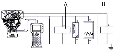
Figure 3-2: Field Wiring for Rosemount 2088 – Low Power Option Code N
