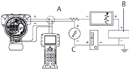
Figure 3-1: Bench Hook-up Wiring Diagrams (4–20 mA Transmitters)
