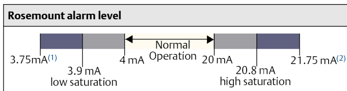
Figure 6-1: Alarm Levels
