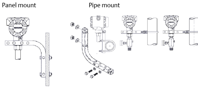
Figure 1-2: Panel and Pipe Mounting
