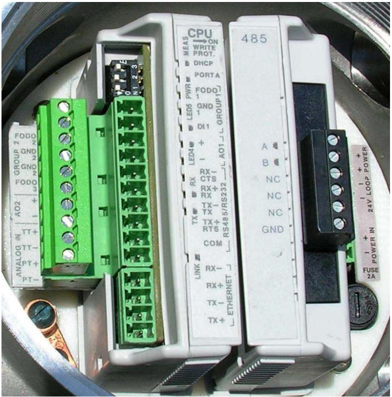
Figure 2-1: 3410/4410 Series Gas Ultrasonic Flow Meter electronics - CPU Module
