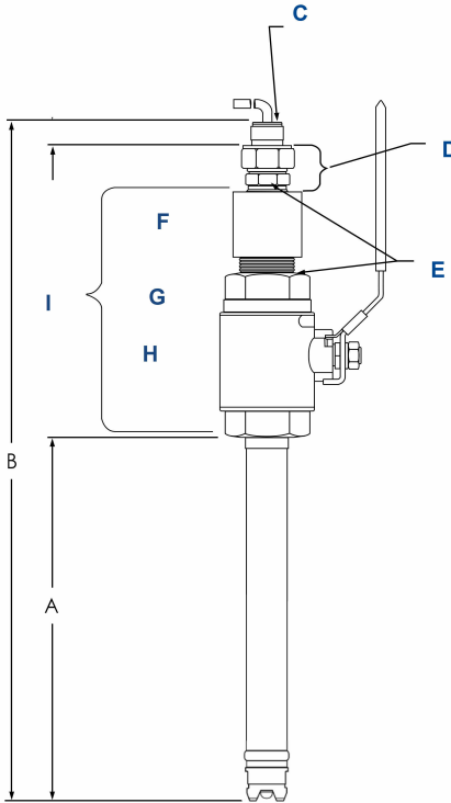
Figure 2-6: RBI Retractable Body Type Sensor (547) with 1½-in. Ball Valve Assembly (PN 23240-00)
