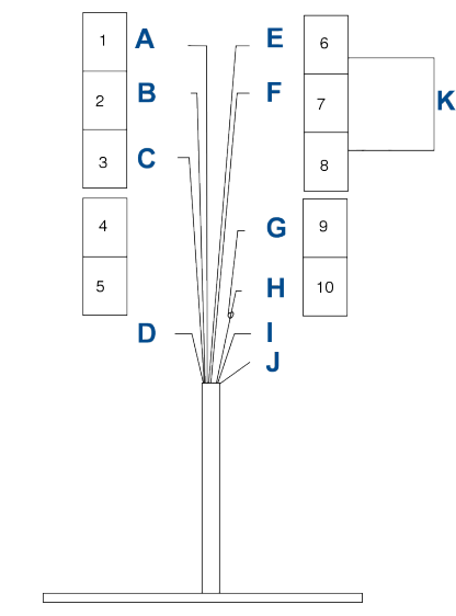
Figure 2-13: Rosemount RBI with Variopol Cable (24281-XX) Wiring Diagram for Rosemount 1066 Transmitters
