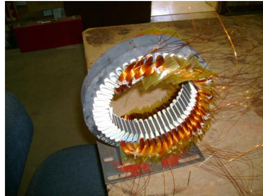
Stator repair
