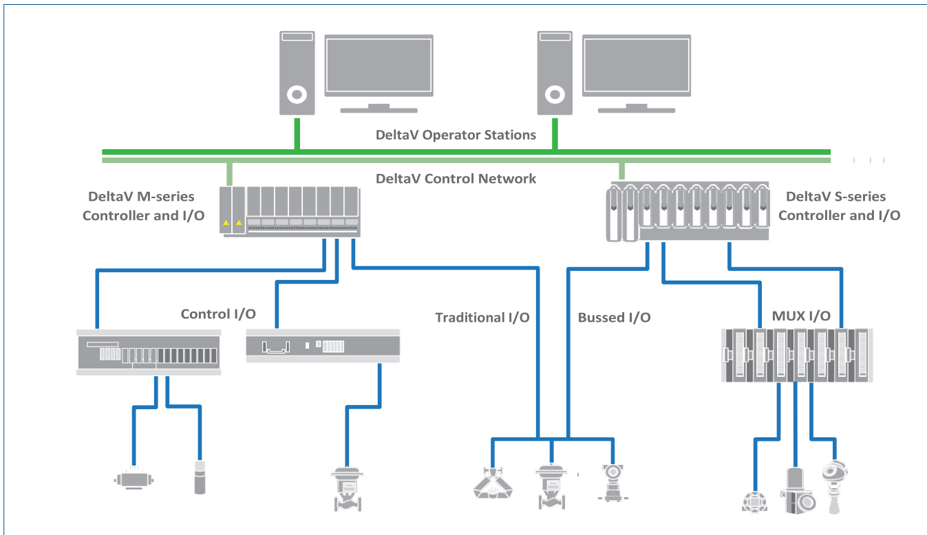
DeltaV™ Flex.CONNECT Solutions for PROVOX™ Control I/O.
