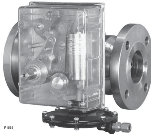
Figure 1. Type BM5/BM5A Slam-Shut Valve
