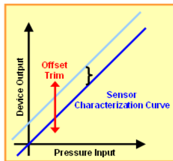
Figure 1-1. Offset Trim
