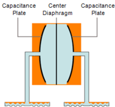
Figure 1-3. Capacitance Pressure Sensor
