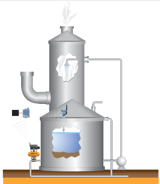
The Fisher 4320 Wireless Position Monitor with On/Off Control Output and Rosemount 2160 Wireless Vibrating Fork Liquid Level Switch were integrated into the DeltaV control logic to provide traditional automation efficiency, but without the traditional cost of engineering and installation of wired instruments and final control elements.
