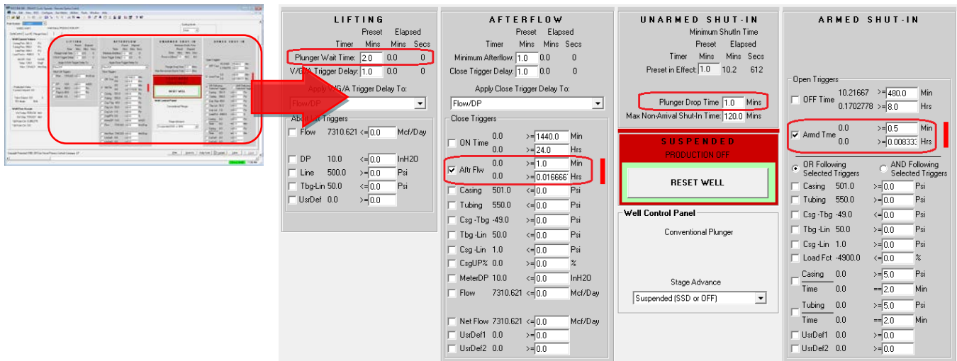
Figure 103. Plunger Lift Simulation – PMWO Cyclic Operate (Plunger Lift Triggers)
