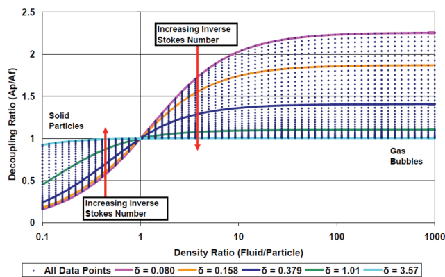
Figure 5: Decoupling Ratio vs. Density Ratio vs. Inverse Stokes number
