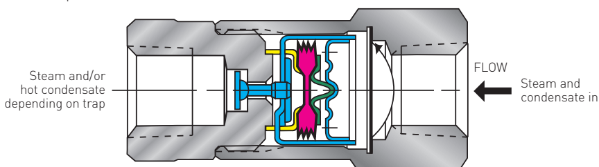
FIGURE 3.11 Bellows trap
