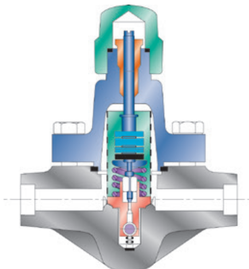
FIGURE 3.10 Bimetallic trap
