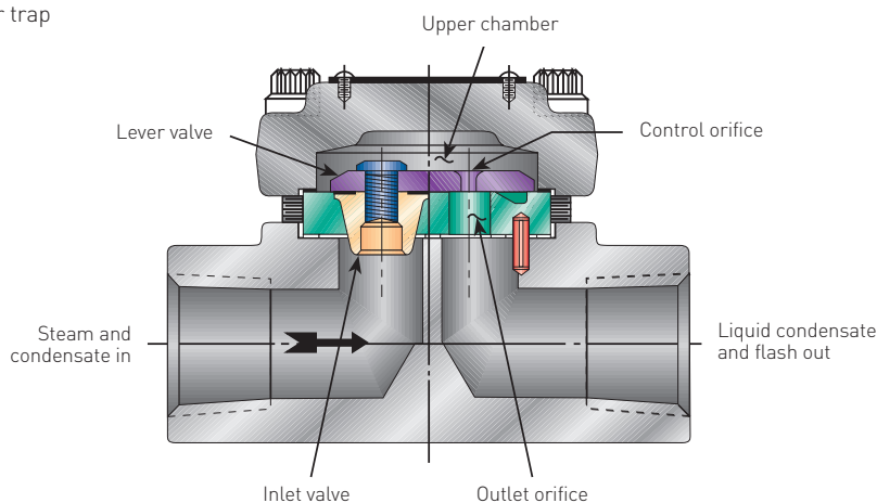
FIGURE 3.3 Lever trap
