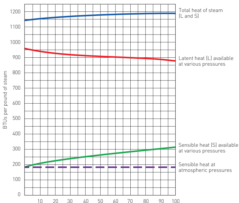
FIGURE 2.4 Saturation curve
